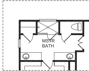
OPTIONAL WALK IN SHOWER
